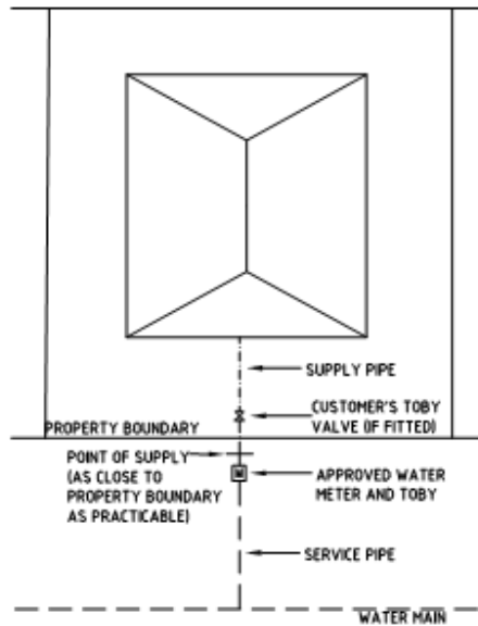
Figure 1: Typical Point of Supply - On Demand Supply - Outside Premises
