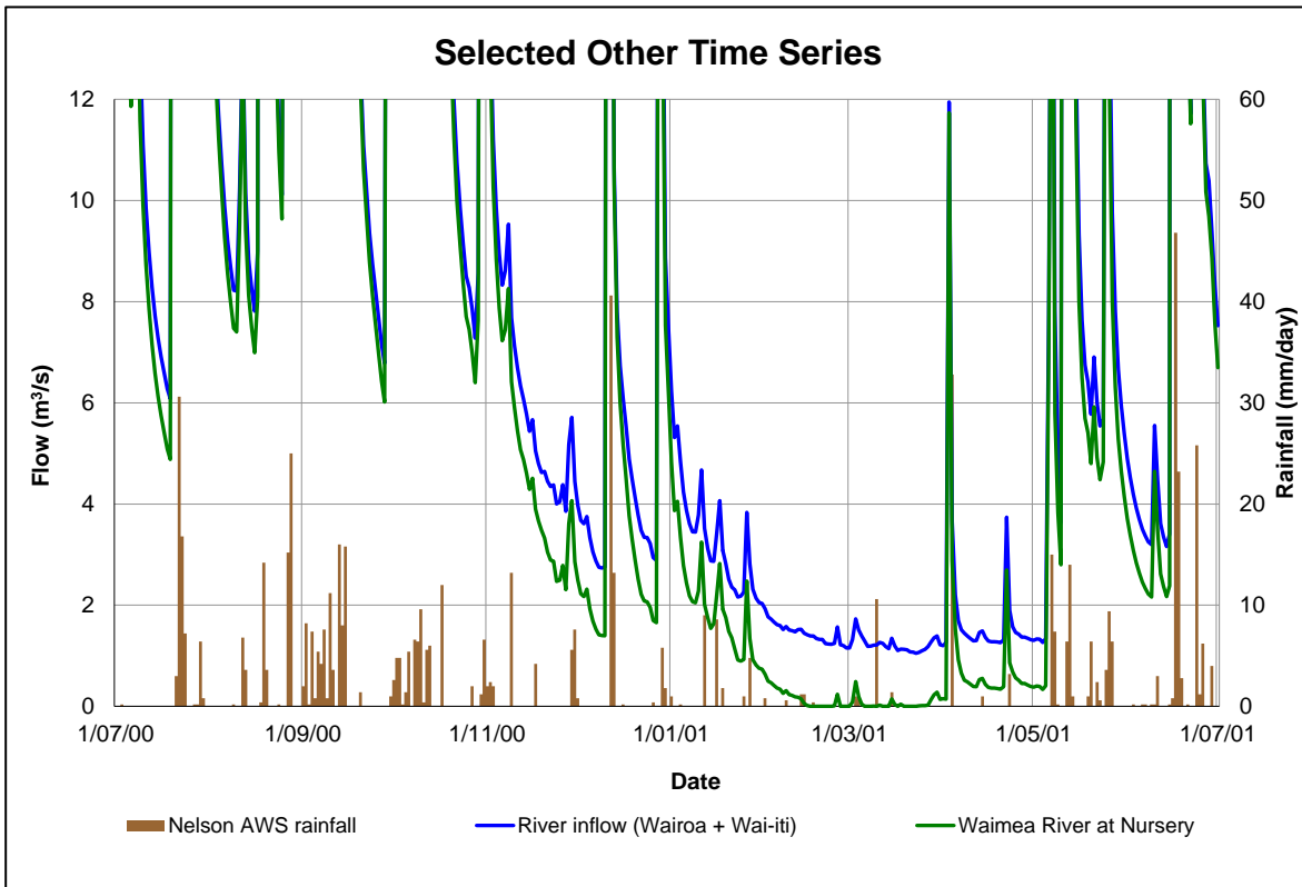
Figure 10: Time series of selected model components: calibration scenario 2000/01
