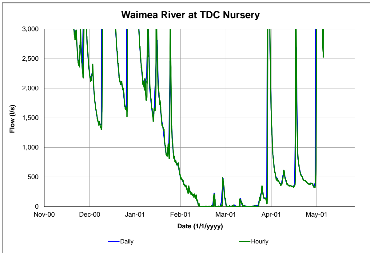
Figure 8: Modelled Nursery river flows comparing daily stresses with hourly river flows and diurnal groundwater pumping
