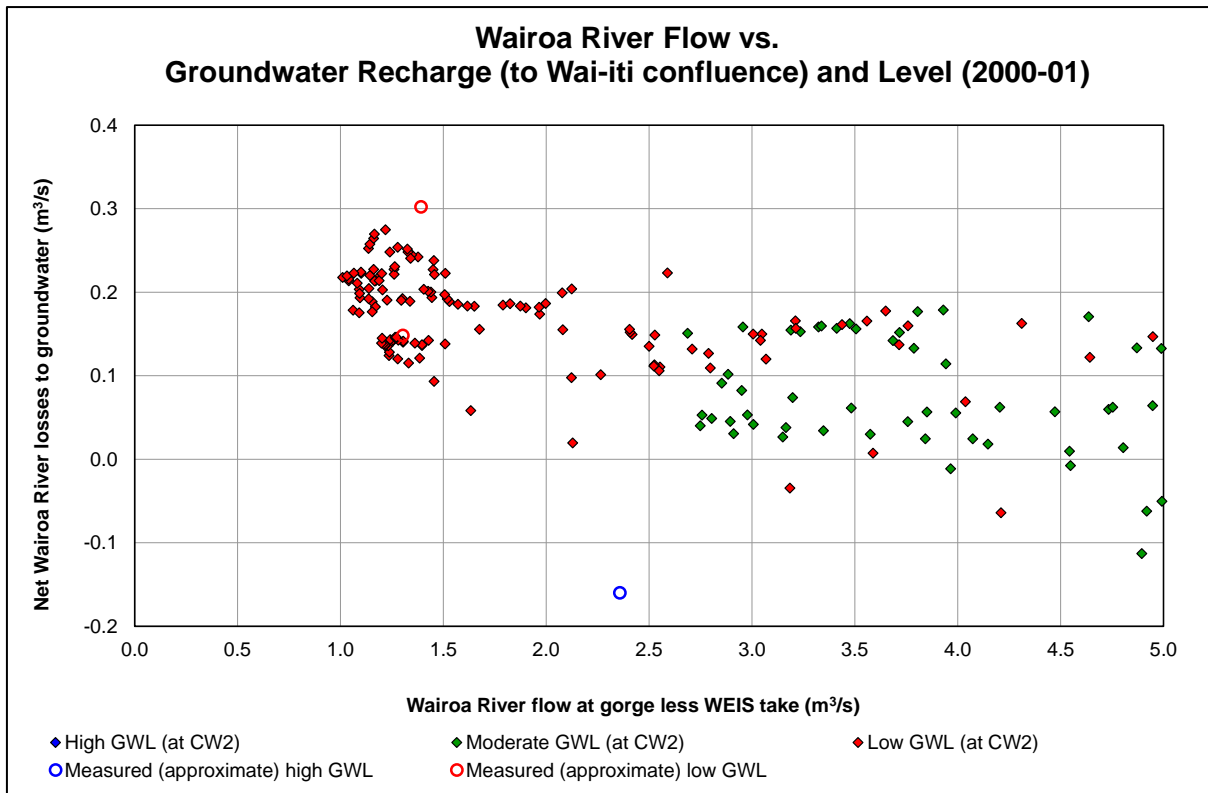
Figure 4: Modelled versus measured Wairoa River losses: low flows
