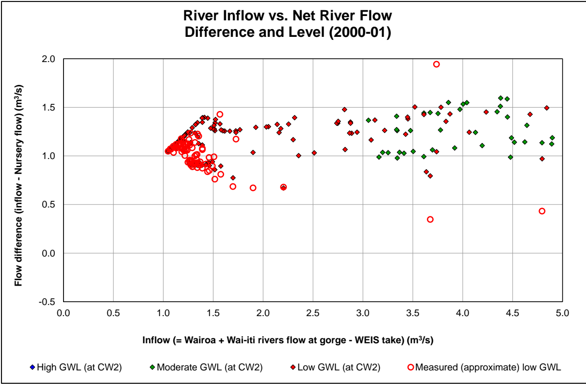
Figure 6: Modelled versus measured Wairoa-Waimea river flow differences: low flows
