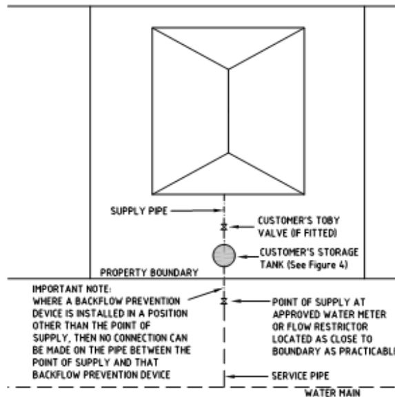
Figure 2: Typical Point of Supply - Restricted Flow Supply - Outside Premises
