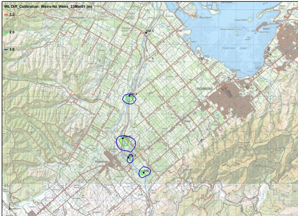
Figure 16: Groundwater level difference due to weirs: Calibration 23 March 2001
