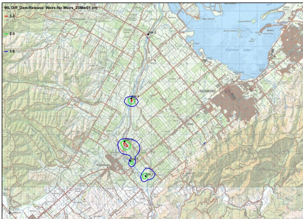
Figure 17: Groundwater level difference due to weirs: Dam release 23 March 2001
