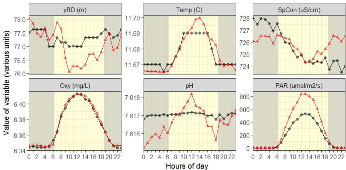
Figure 3-7: Diurnal variability of visibility estimates in comparison to other water quality variables over the 3-month deployment. Top panels, left to right, are for visual clarity, temperature, and specific conductance. Bottom panels, left to right, are for dissolved oxygen, pH and sunlight (photosynthetically available radiation; PAR). Note: Medians (grey circles) and means (red triangles) were calculated over the entire dataset, after day median normalisation of each variable to maximise diurnal signals between days with changes in variable magnitude.
