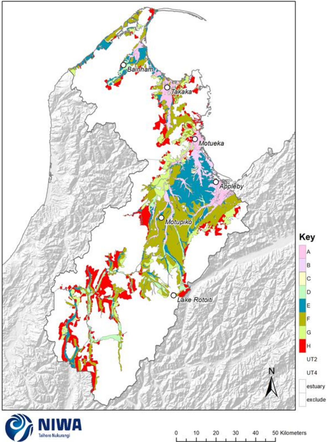
Figure 9-1: Land classes of Tasman District. Refer to Table 9-1 for interpretation of each land class. Note that 'exclude' refers to land that is excluded from this classification system as it is conservation land. After Agriculture New Zealand (1994)
