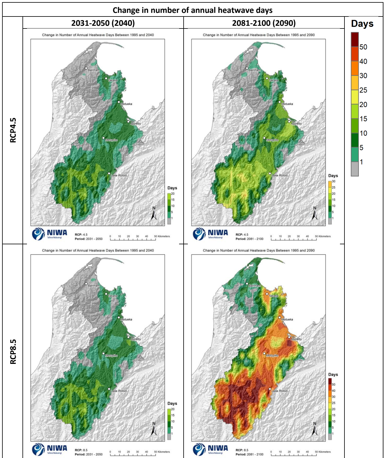
Figure 3-2: Projected annual heatwave day changes (number of days within periods of \geq three consecutive days with maximum temperatures > 25^\circ\text{C} ) at 2040 and 2090. Relative to 1986-2005 average, for RCP4.5 and RCP8.5, based on the average of six global climate models. Results are based on dynamical downscaled projections using NIWA's Regional Climate Model. Resolution of projection is 5km x 5km.
