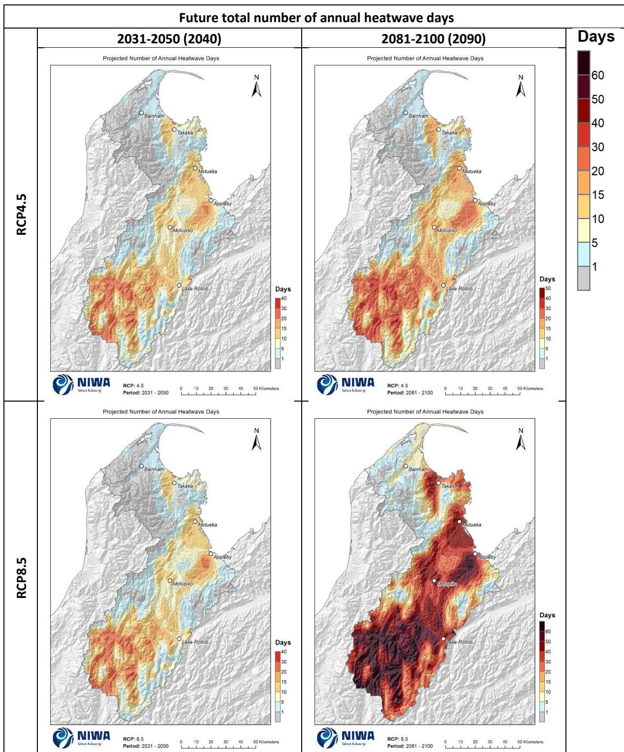
Figure 3-3: Projected annual total number of heatwave days (number of days within periods of \geq three consecutive days with maximum temperatures > 25^{\circ}\text{C} ) at 2040 and 2090. For RCP4.5 and RCP8.5, based on the average of six global climate models. Results are based on dynamical downscaled projections using NIWA's Regional Climate Model. Resolution of projection is 5km x 5km.
