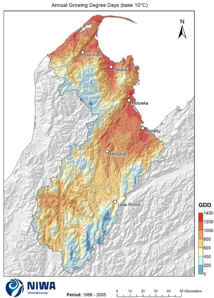
Figure 4-1: Modelled annual number of growing degree days (base 10°C), average over the historic period 1986-2005. Results are based on dynamical downscaled projections using NIWA's Regional Climate Model. Resolution of projection is 5km x 5km.
