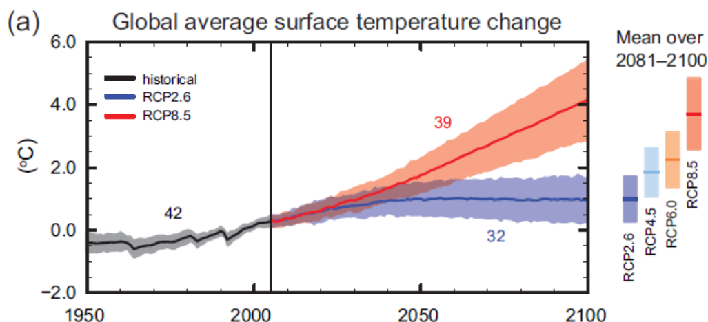
Figure 11-2: CMIP5 multi-model simulated time series from 1950-2100 for change in global annual mean surface temperature relative to 1986-2005. Time series of projections and a measure of uncertainty (shading) are shown for scenarios RCP2.6 (blue) and RCP8.5 (red). Black (grey shading) is the modelled historical evolution using historical reconstructed forcings. The mean and associated uncertainties averaged over 2081-2100 are given for all RCP scenarios as coloured vertical bars to the right of the graph (the mean projection is the solid line in the middle of the bars). The numbers of CMIP5 models used to calculate the multi-model mean is indicated on the graph. From IPCC (2013).
