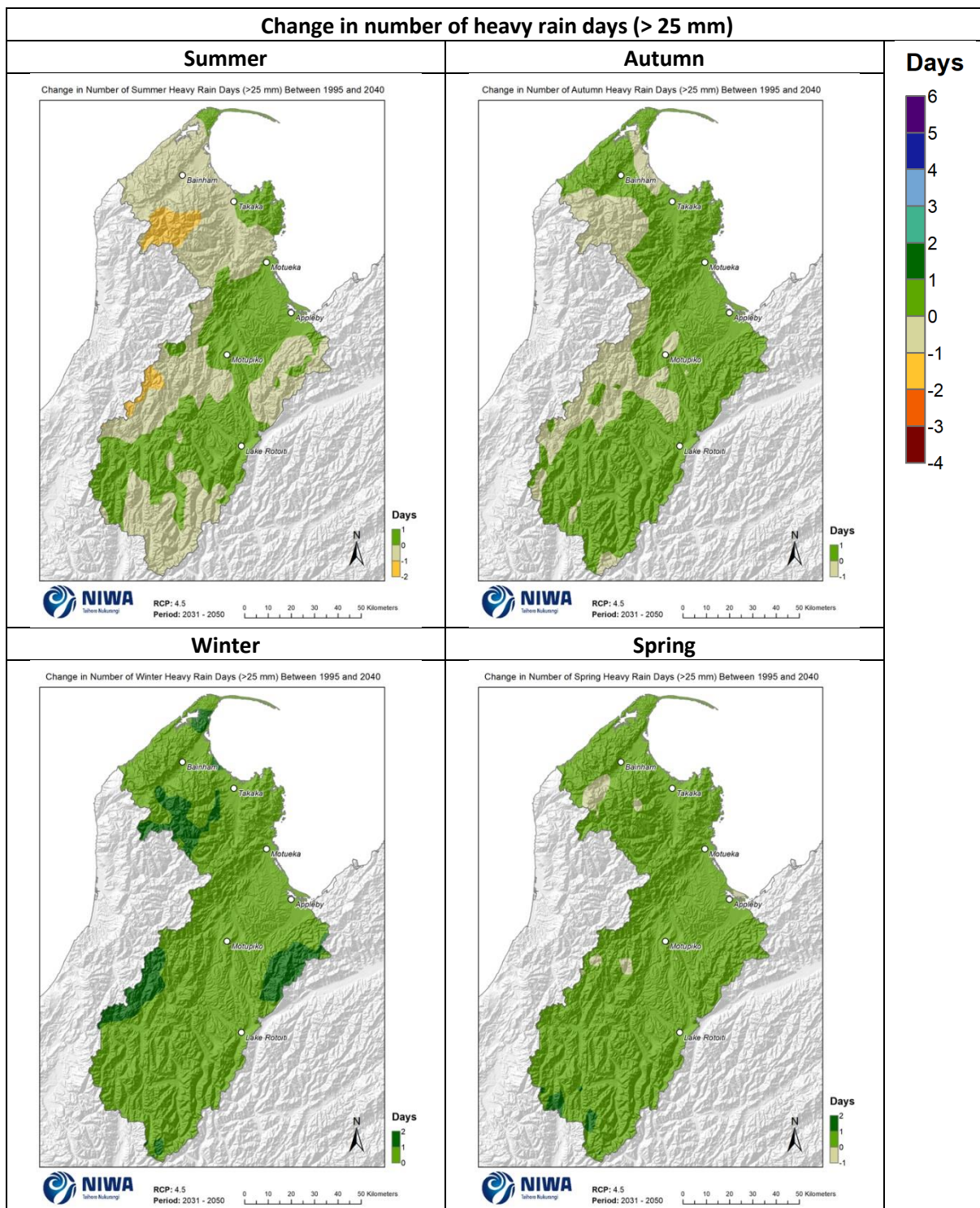
Figure 5-4: Projected change in seasonal number of heavy rain days (>25mm) by 2040 for RCP4.5. Relative to 1986-2005 average, based on the average of six global climate models. Results are based on dynamical downscaled projections using NIWA's Regional Climate Model. Resolution of projection is 5km x 5km.
