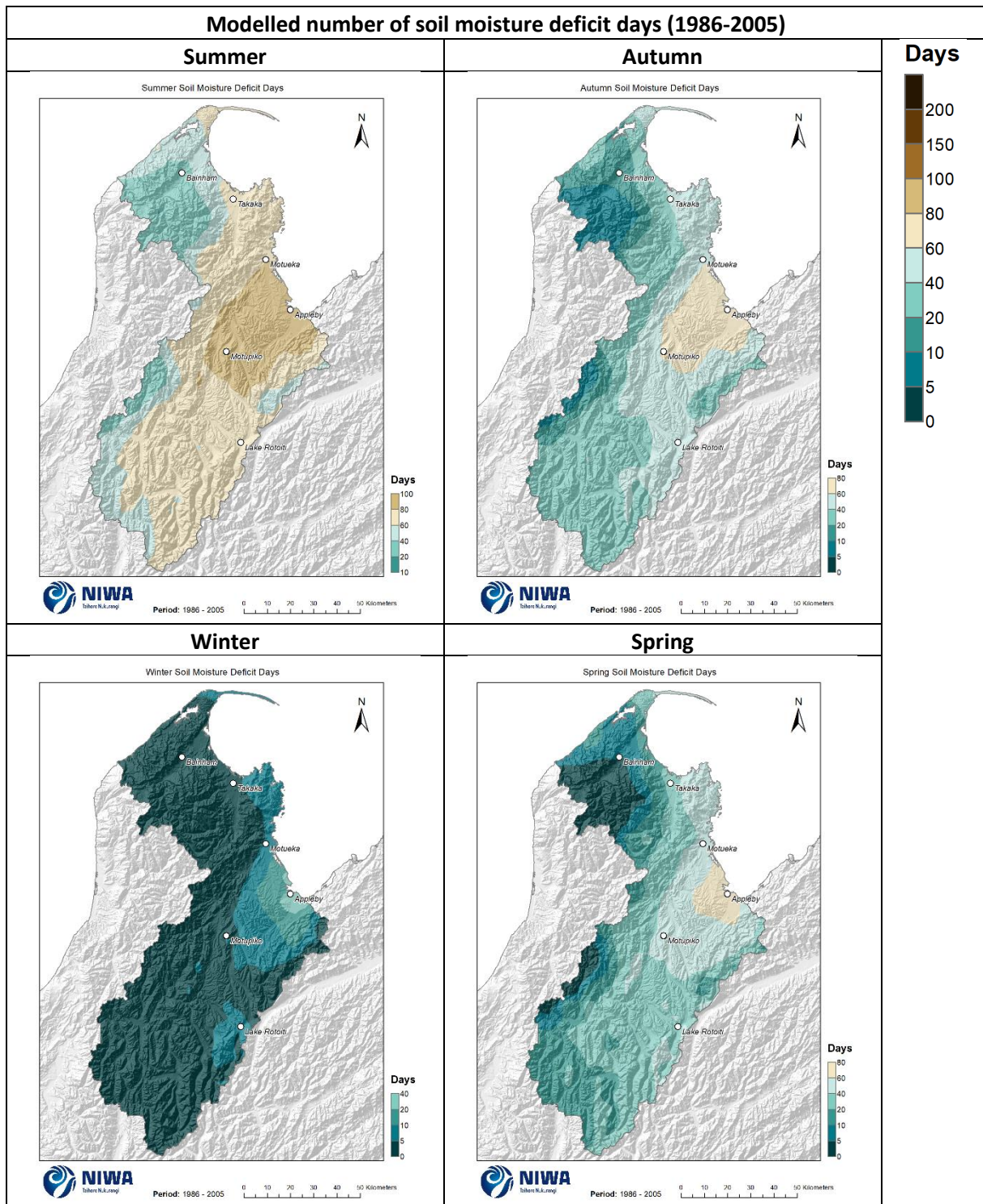
Figure 8-2: Modelled seasonal number of days of soil moisture deficit (average over the historic period 1986-2005). Based on the average of six global climate models. Results are based on dynamical downscaled projections using NIWA's Regional Climate Model. Resolution of projection is 5km x 5km.
