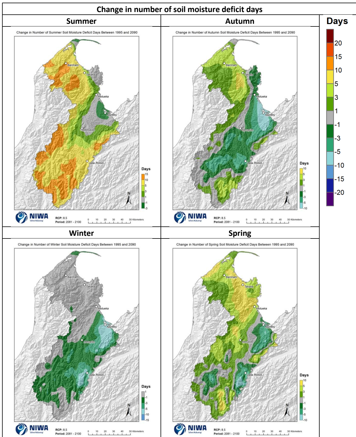
Figure 8-10: Projected change in seasonal number of days of soil moisture deficit by 2090 for RCP8.5. Relative to 1986–2005 average, based on the average of six global climate models. Results are based on dynamical downscaled projections using NIWA's Regional Climate Model. Resolution of projection is 5km x 5km.
