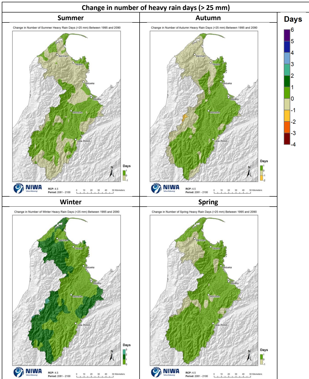
Figure 5-8: Projected change in seasonal number of heavy rain days (>25mm) by 2090 for RCP4.5. Relative to 1986-2005 average, based on the average of six global climate models. Results are based on dynamical downscaled projections using NIWA's Regional Climate Model. Resolution of projection is 5km x 5km.
