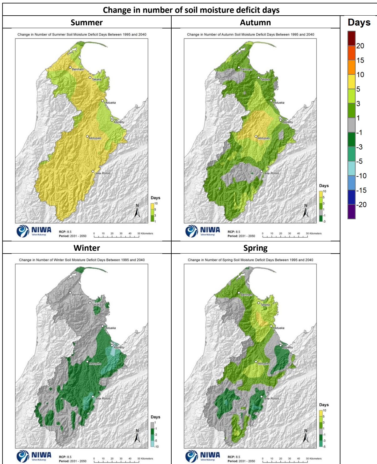
Figure 8-6: Projected change in seasonal number of days of soil moisture deficit by 2040 for RCP8.5. Relative to 1986-2005 average, based on the average of six global climate models. Results are based on dynamical downscaled projections using NIWA's Regional Climate Model. Resolution of projection is 5km x 5km.
