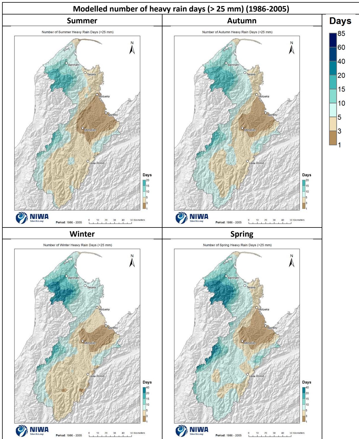
Figure 5-2: Modelled seasonal number of heavy rain days (>25mm) (average over the historic period 1986-2005). Based on the average of six global climate models. Results are based on dynamical downscaled projections using NIWA's Regional Climate Model. Resolution of projection is 5km x 5km.
