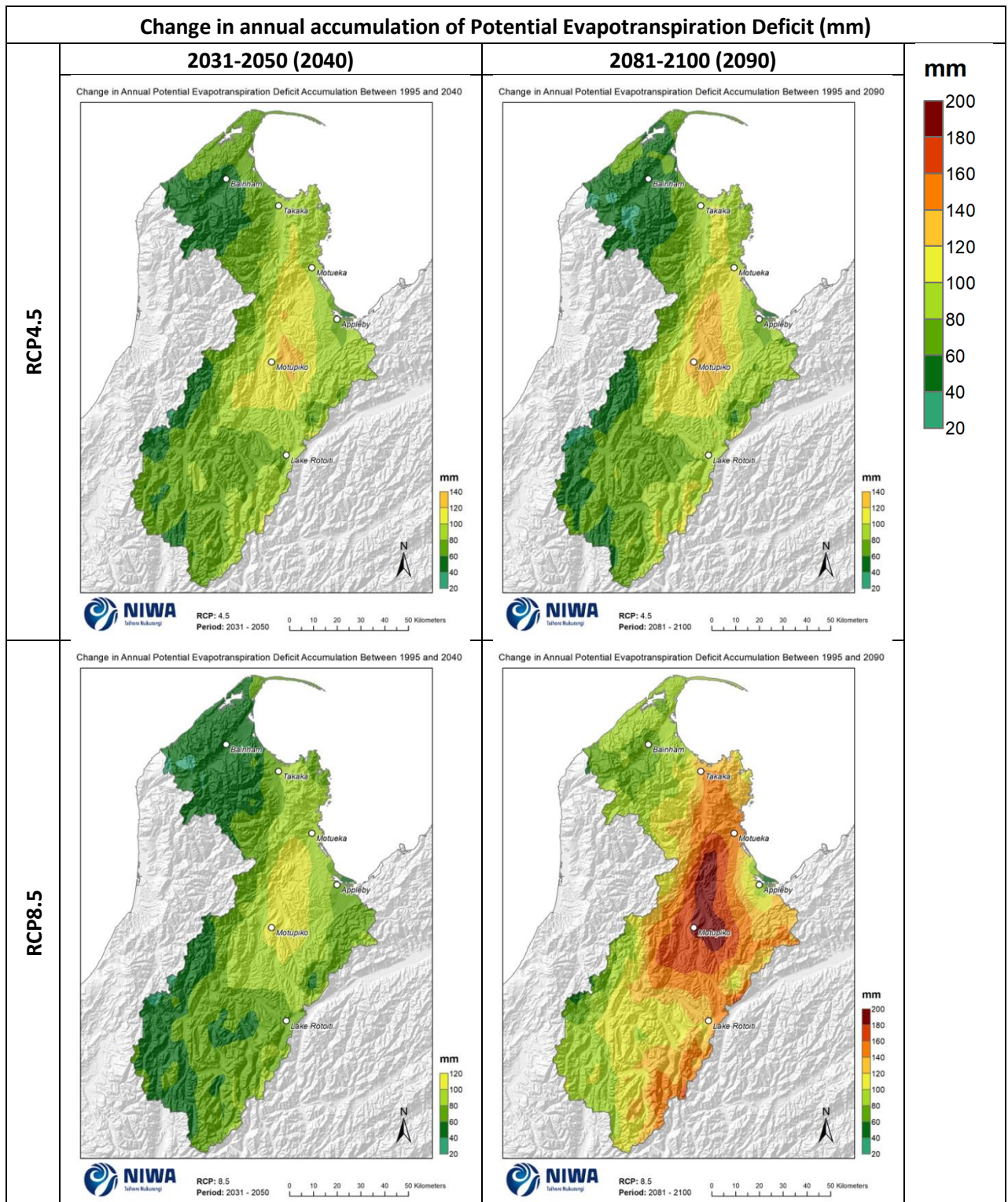
Figure 7-2: Projected annual change in accumulated Potential Evapotranspiration Deficit (mm) at 2040 and 2090. Relative to 1986-2005 average, for RCP4.5 and RCP8.5, based on the average of six global climate models. Results are based on dynamical downscaled projections using NIWA's Regional Climate Model. Resolution of projection is 5km x 5km.
