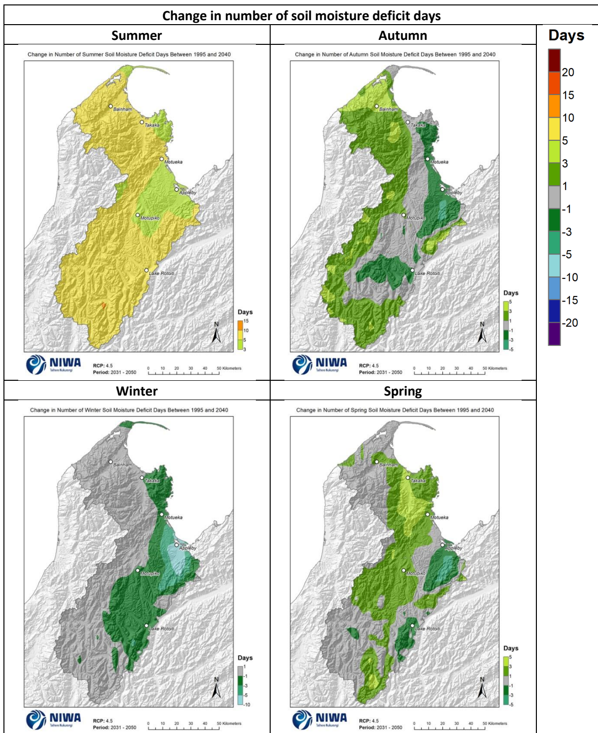
Figure 8-4: Projected change in seasonal number of days of soil moisture deficit by 2040 for RCP4.5. Relative to 1986-2005 average, based on the average of six global climate models. Results are based on dynamical downscaled projections using NIWA's Regional Climate Model. Resolution of projection is 5km x 5km.
