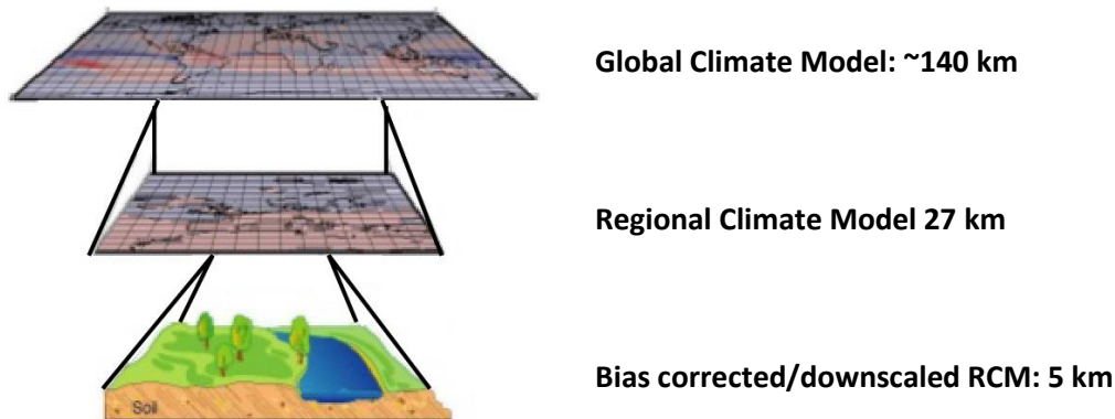
Figure 11-1: Schematic showing dynamical downscaling method used in this report.
