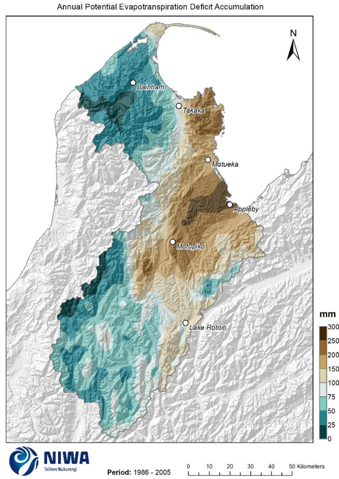
Figure 7-1: Modelled annual accumulated Potential Evapotranspiration Deficit (mm), average over 1986-2005. Results are based on dynamical downscaled projections using NIWA's Regional Climate Model. Resolution of projection is 5km x 5km.
