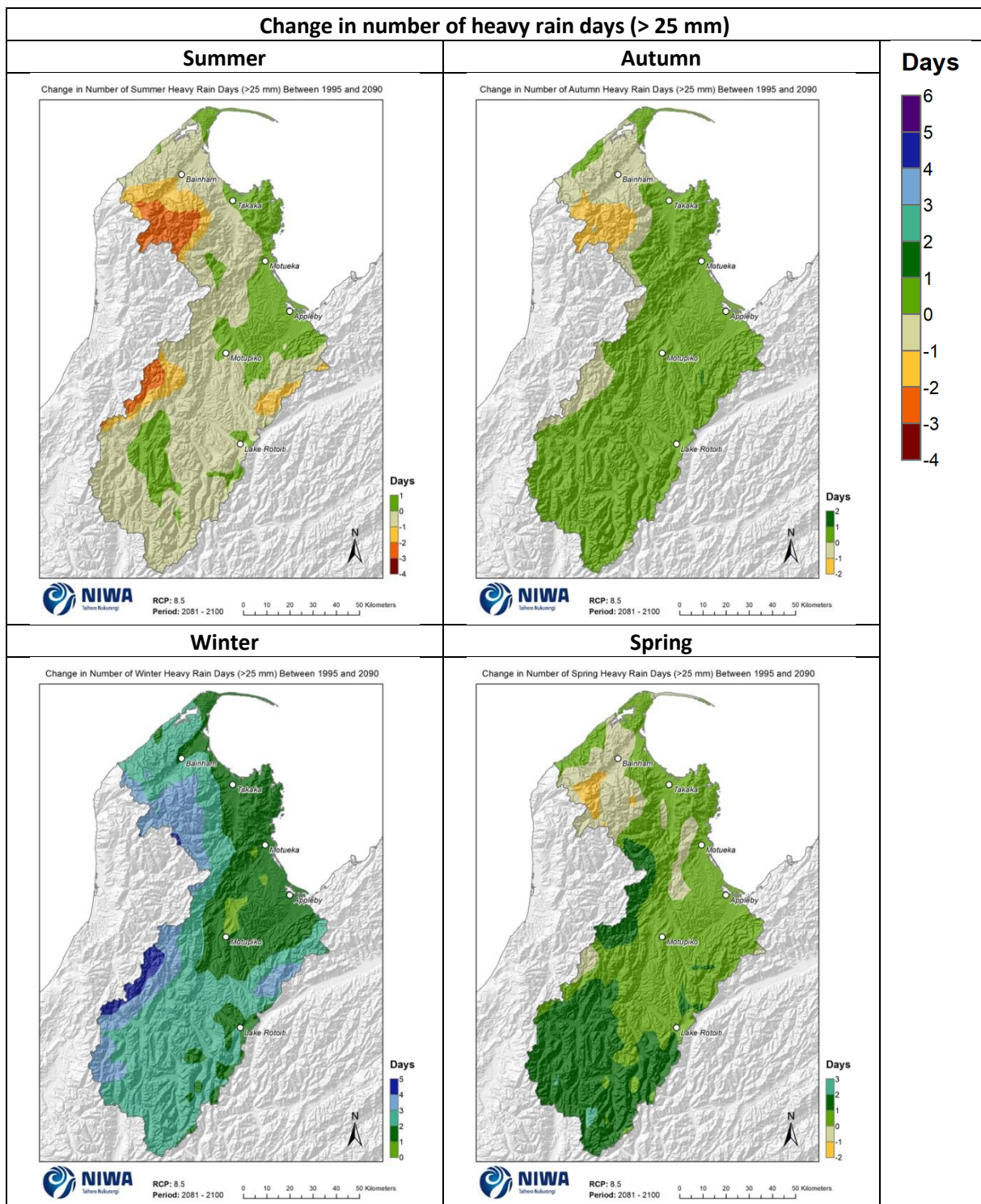
Figure 5-10: Projected change in seasonal number of heavy rain days (>25mm) by 2090 for RCP8.5. Relative to 1986-2005 average, based on the average of six global climate models. Results are based on dynamical downscaled projections using NIWA's Regional Climate Model. Resolution of projection is 5km x 5km.
