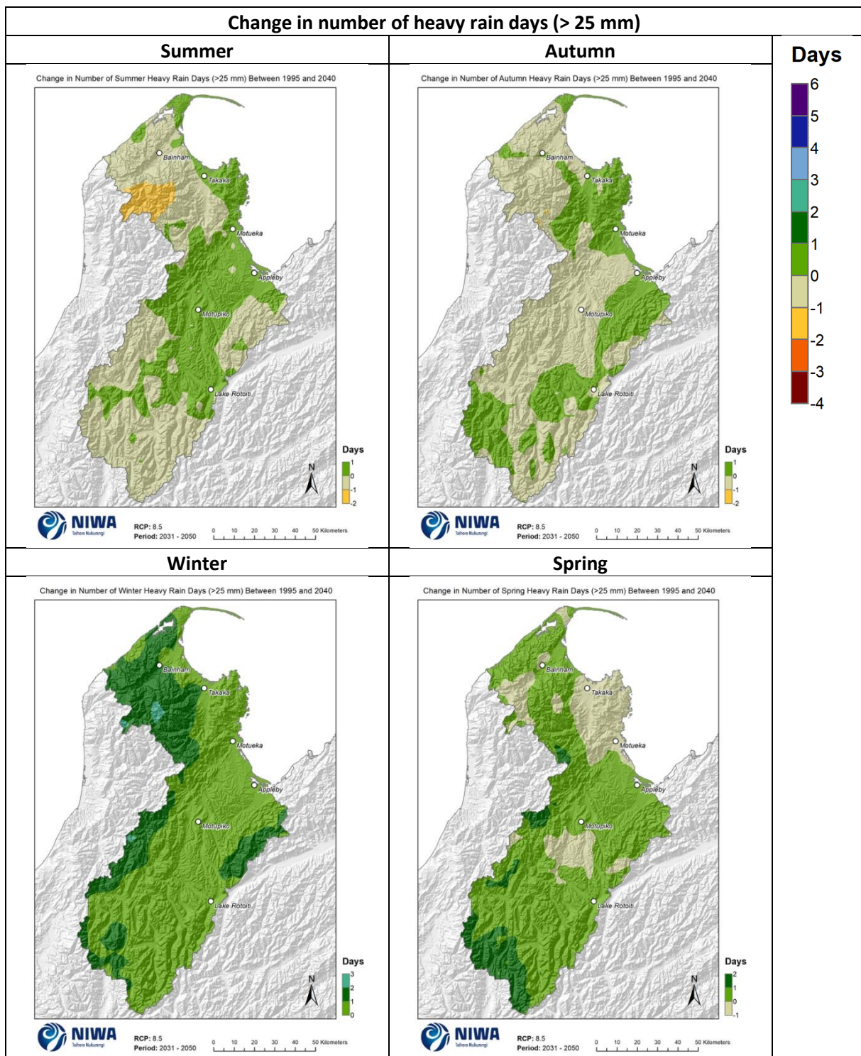
Figure 5-6: Projected change in seasonal number of heavy rain days (>25mm) by 2040 for RCP8.5. Relative to 1986-2005 average, based on the average of six global climate models. Results are based on dynamical downscaled projections using NIWA's Regional Climate Model. Resolution of projection is 5km x 5km.
