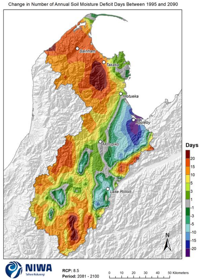
Figure 8-9: Projected change in annual number of days of soil moisture deficit by 2090 for RCP8.5. Relative to 1986-2005 average, based on the average of six global climate models. Results are based on dynamical downscaled projections using NIWA's Regional Climate Model. Resolution of projection is 5km x 5km.
