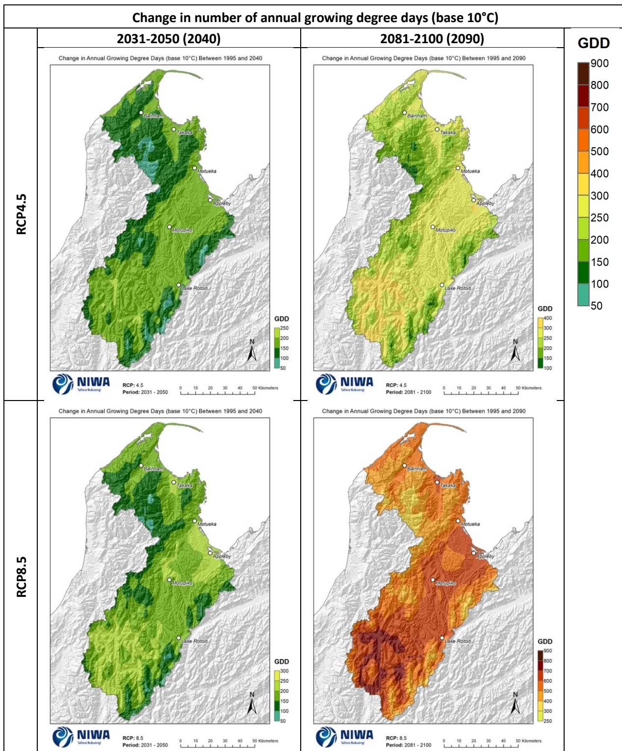
Figure 4-2: Projected annual growing degree day changes (base 10°C) at 2040 and 2090. Relative to 1986-2005 average, for RCP4.5 and RCP8.5, based on the average of six global climate models. Results are based on dynamical downscaled projections using NIWA's Regional Climate Model. Resolution of projection is 5km x 5km.
