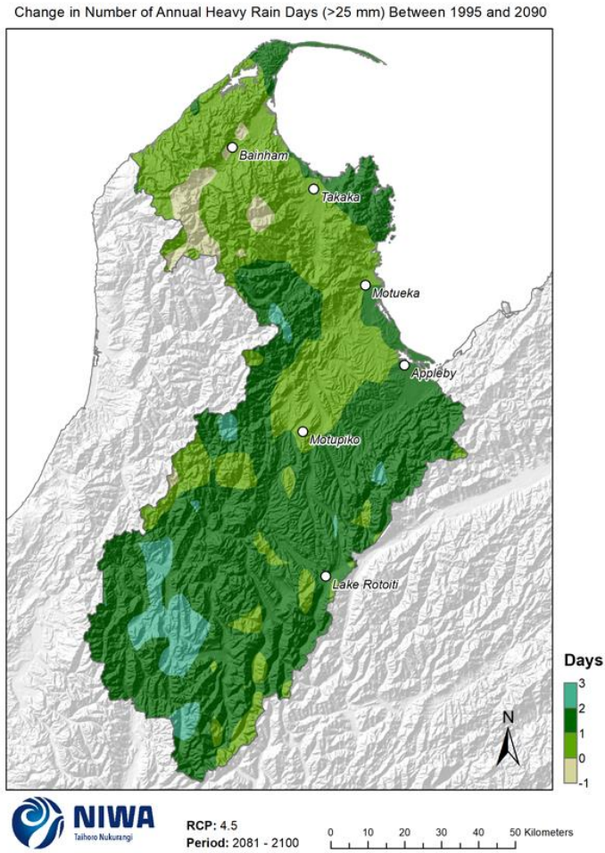
Figure 5-7: Projected change in annual number of heavy rain days (>25mm) by 2090 for RCP4.5. Relative to 1986-2005 average, based on the average of six global climate models. Results are based on dynamical downscaled projections using NIWA's Regional Climate Model. Resolution of projection is 5km x 5km.
