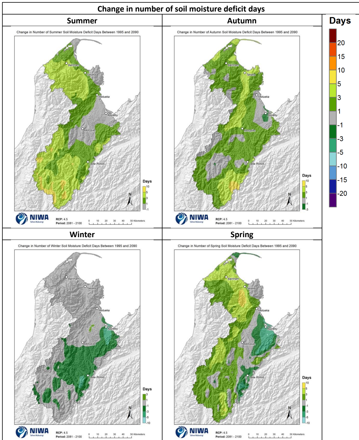
Figure 8-8: Projected change in seasonal number of days of soil moisture deficit by 2090 for RCP4.5. Relative to 1986-2005 average, based on the average of six global climate models. Results are based on dynamical downscaled projections using NIWA's Regional Climate Model. Resolution of projection is 5km x 5km.
