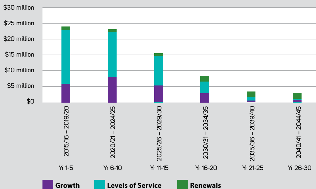
Fig 17 Years 1-30: Stormwater 5 yearly capital expenditure totals
