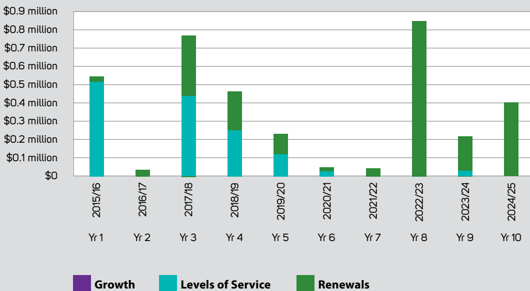
Fig 36 Years 1-10: Solid Waste annual capital expenditure
