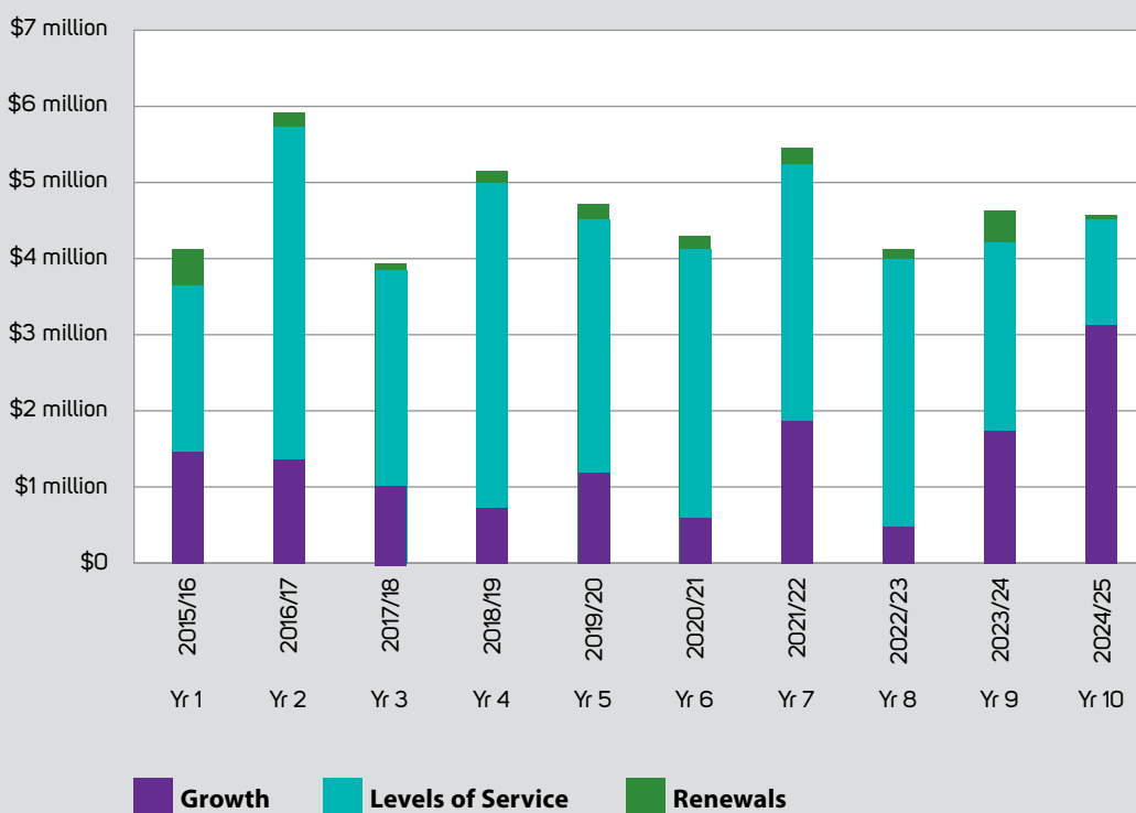
Fig 16 Years 1-10: Stormwater annual capital expenditure
