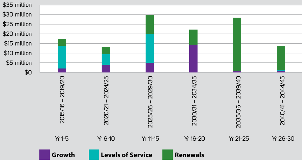
Fig 22 Years 1-30: Wastewater 5 yearly capital expenditure totals
